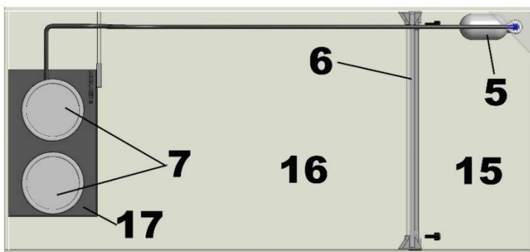
Fig. 1a: Filter sump Armatus Lagoon 400
