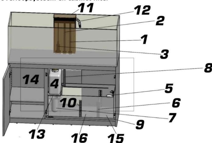
Fig. 1: Overloop en cabinet filter
