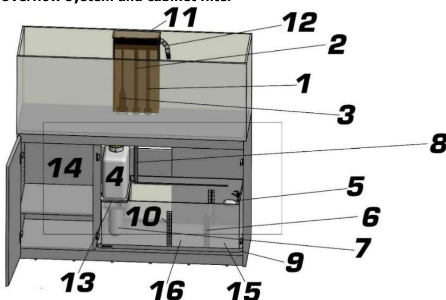
Fig. 1: Overflow and cabinet filter
